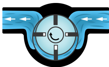
Vingepumpe, prinsipp
